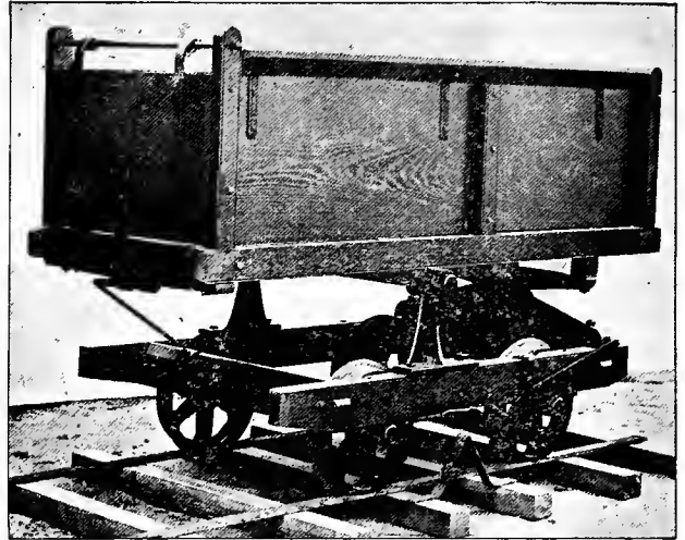
Fig. 29. MINE CAR, AUTOMATIC END DUMP, BUILT BY C. W. RAYMOND & CO.
